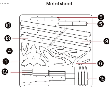
Metal sheet
